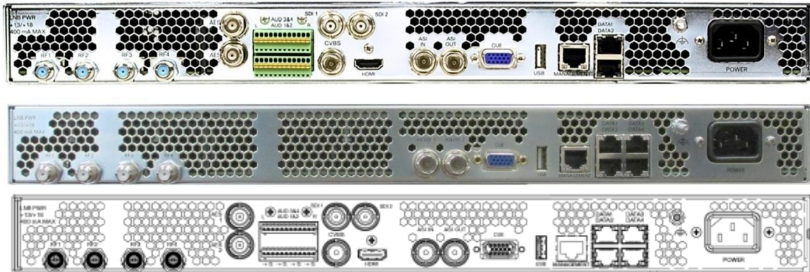
Figure 2. Synamedia PowerVu Professional Receiver rear panel
